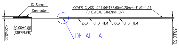
FPC assembling suggestion
